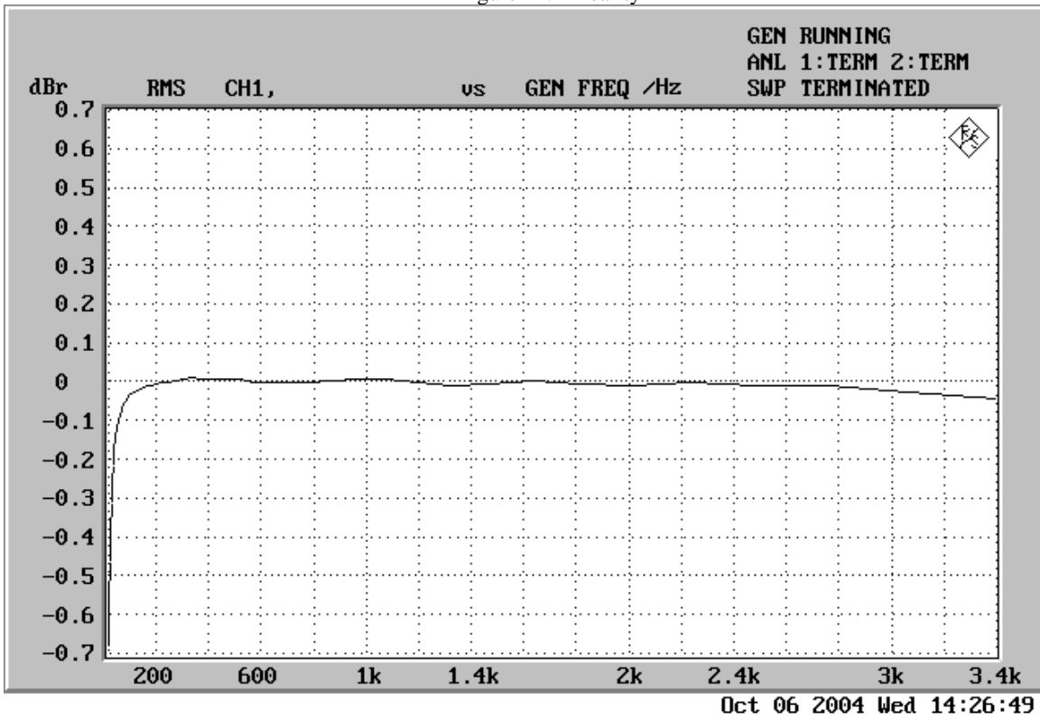
Figure 13. Frequency Response
