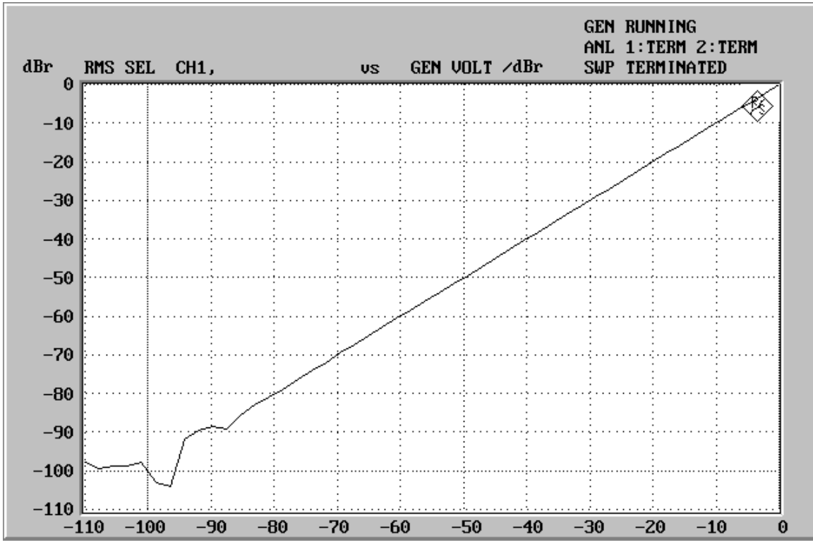
Figure 12. Linearity
